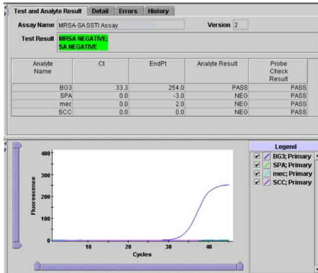
Figure 4. An example of a MRSA negative/SA negative result
